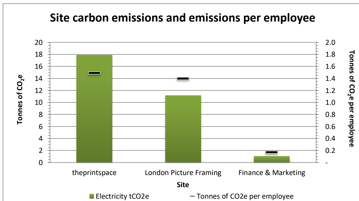
Figure 4: CO 2 e emissions on a per site and employee basis
